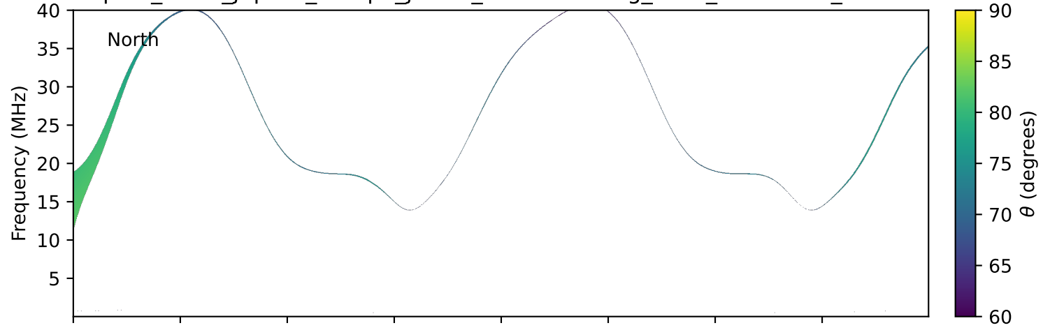
expres_earth_jupiter_europa_jrm33_lossc-wid1deg_3kev_19931215_v11.cdf
