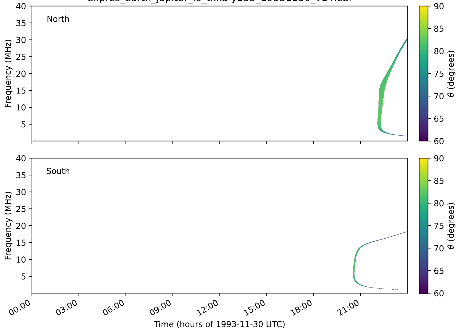
expres_earth_jupiter_io_txka-y235_19931130_v14.cdf
