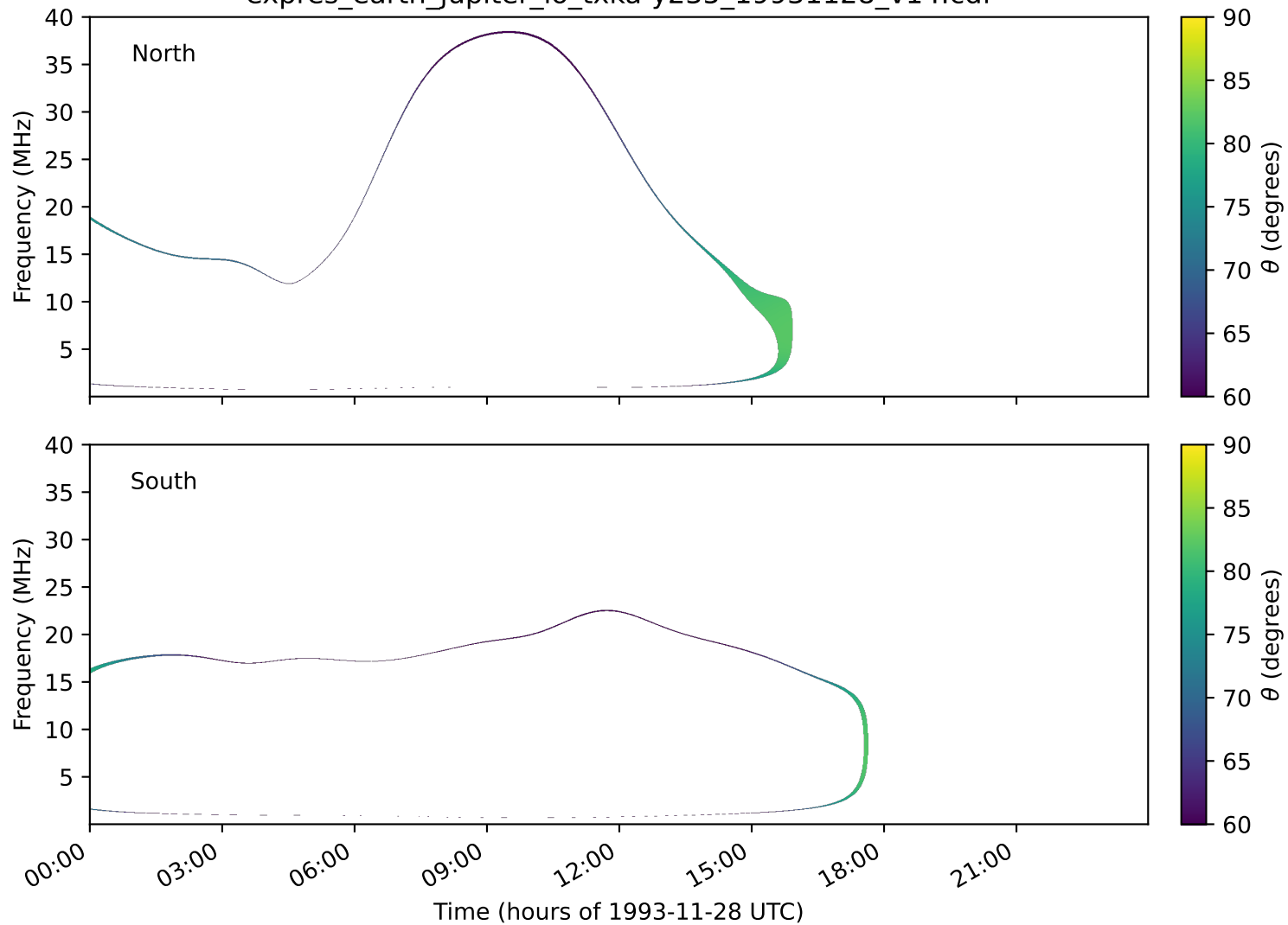
expres_earth_jupiter_io_txka-y235_19931128_v14.cdf
