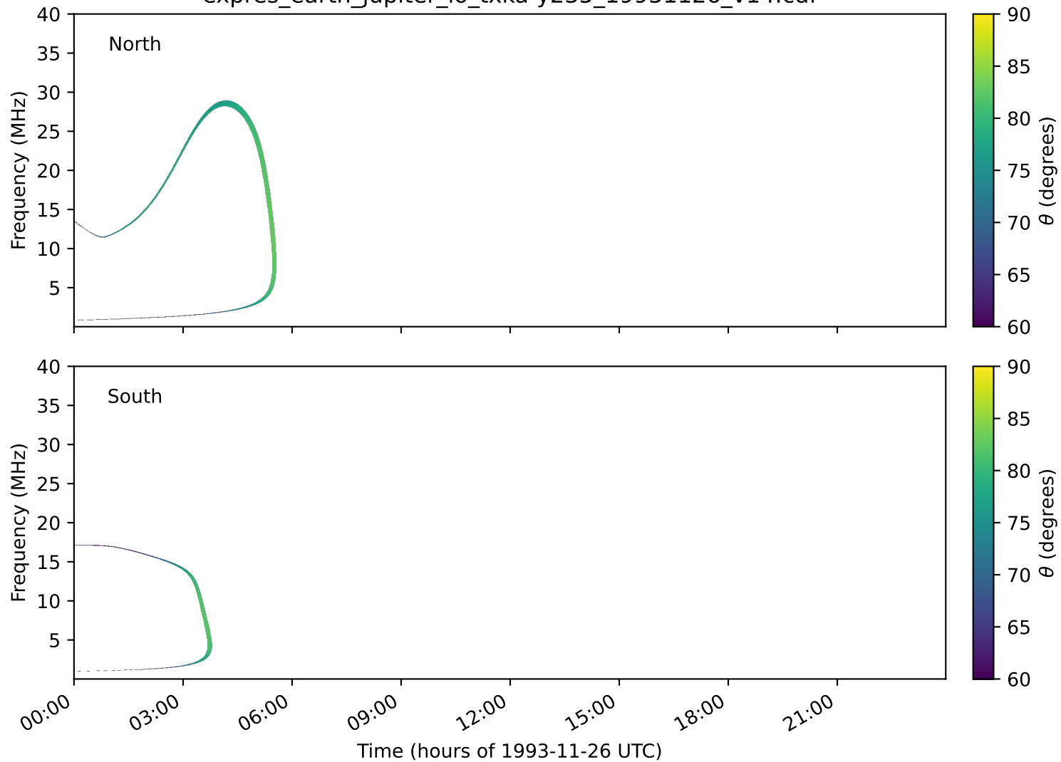
expres_earth_jupiter_io_txka-y235_19931126_v14.cdf
