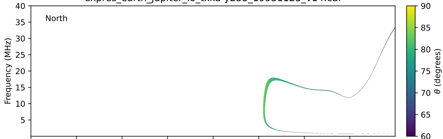
expres_earth_jupiter_io_txka-y235_19931123_v14.cdf
