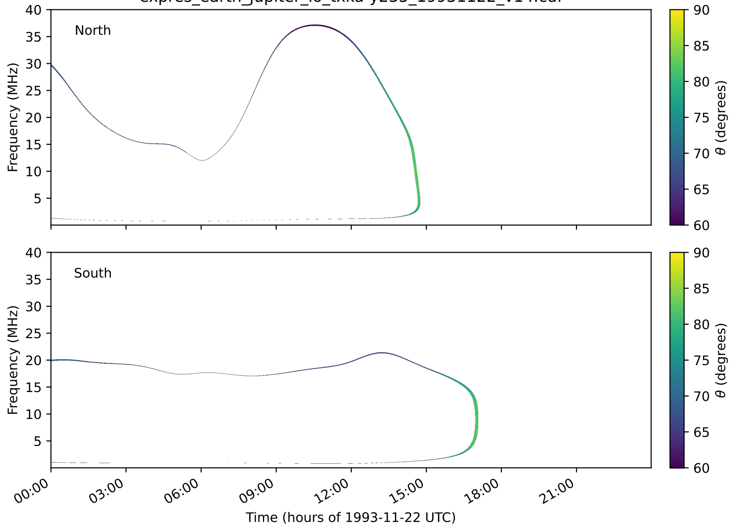
expres_earth_jupiter_io_txka-y235_19931122_v14.cdf
