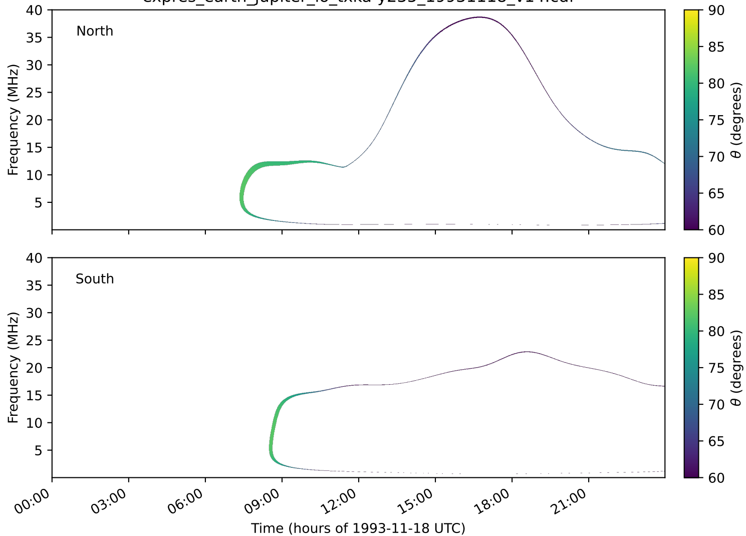
expres_earth_jupiter_io_txka-y235_19931118_v14.cdf
