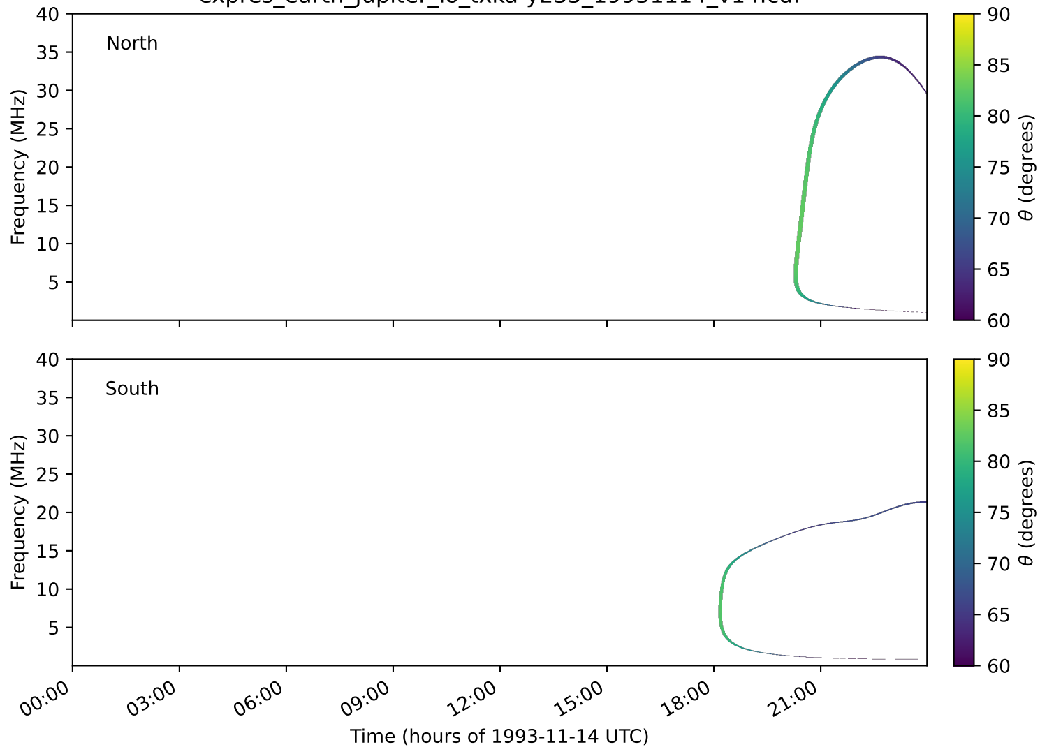
expres_earth_jupiter_io_txka-y235_19931114_v14.cdf
