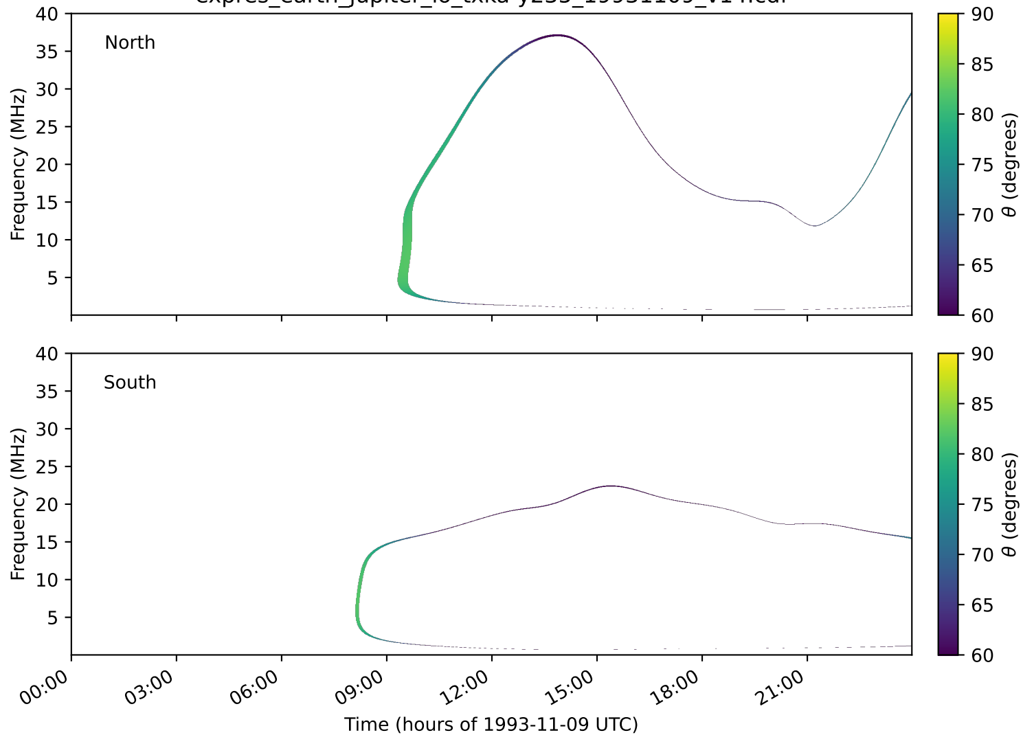
expres_earth_jupiter_io_txka-y235_19931109_v14.cdf
