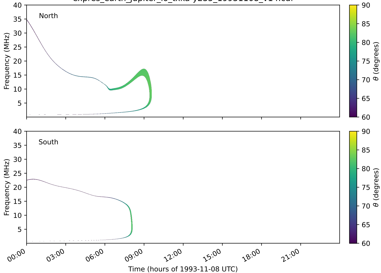
expres_earth_jupiter_io_txka-y235_19931108_v14.cdf
