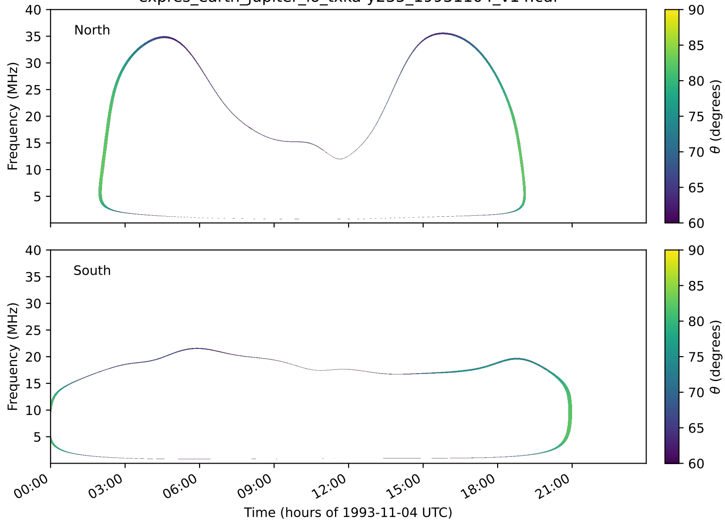
expres_earth_jupiter_io_txka-y235_19931104_v14.cdf
