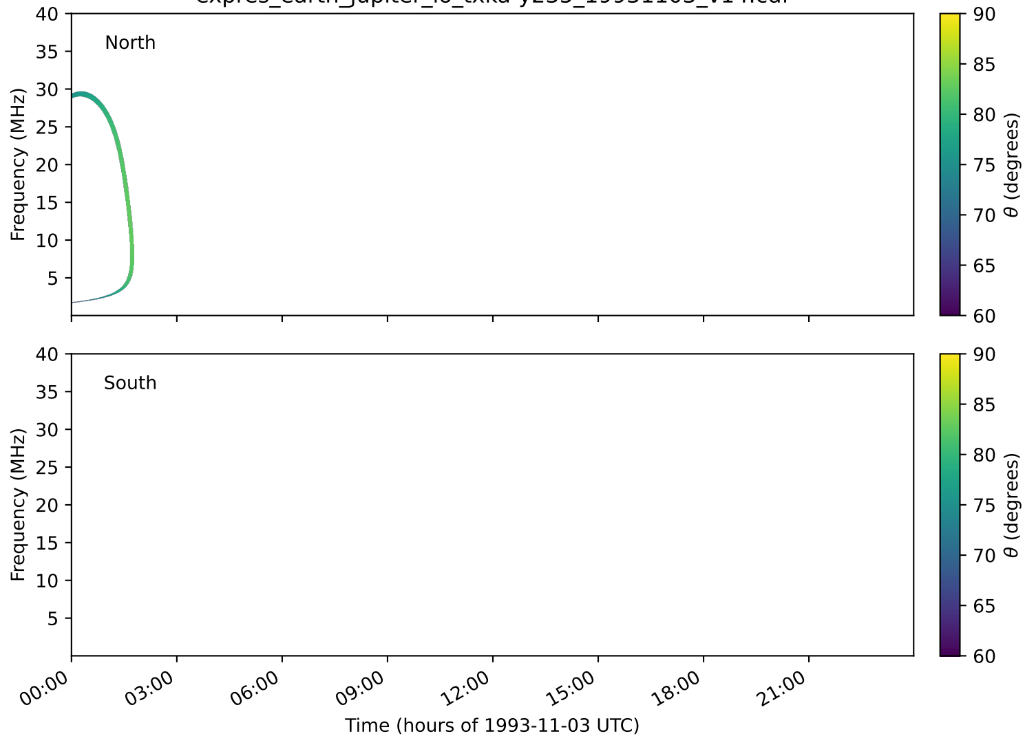
expres_earth_jupiter_io_txka-y235_19931103_v14.cdf
