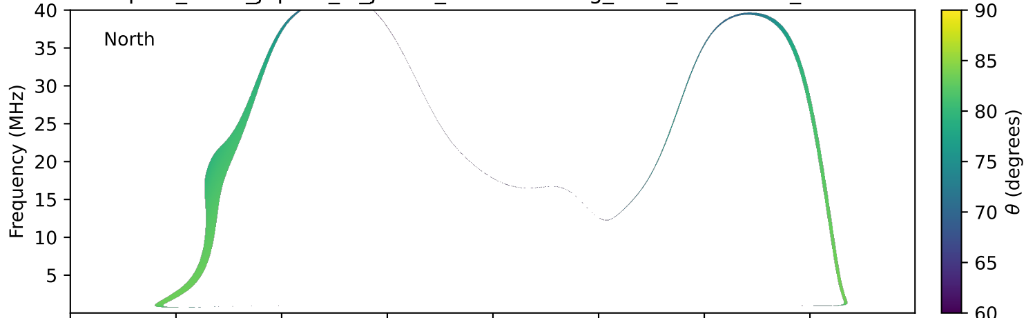
expres_earth_jupiter_io_jrm33_lossc-wid1deg_3kev_19931120_v11.cdf
