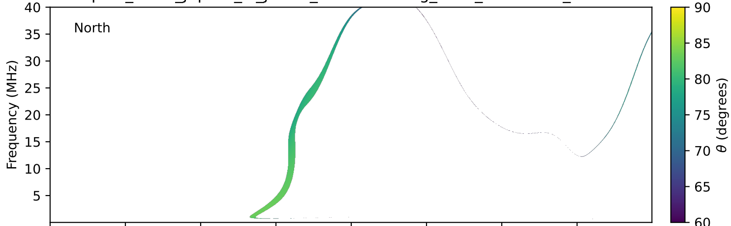
expres_earth_jupiter_io_jrm33_lossc-wid1deg_3kev_19931109_v11.cdf
