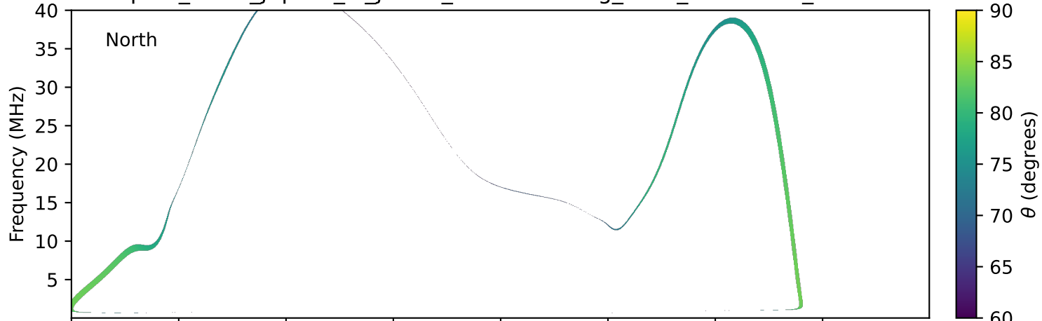
expres_earth_jupiter_io_jrm09_lossc-wid1deg_3kev_19931113_v11.cdf
