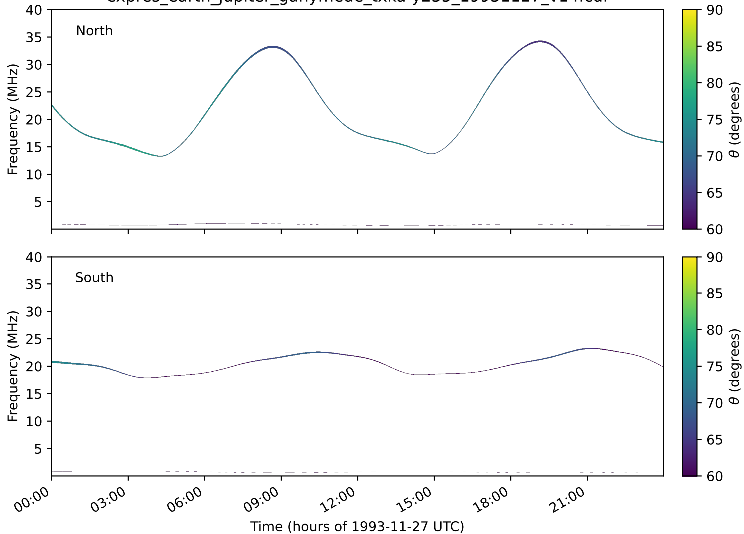
expres_earth_jupiter_ganymede_txka-y235_19931127_v14.cdf
