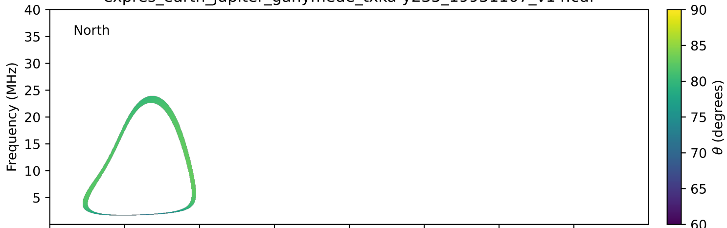
expres_earth_jupiter_ganymede_txka-y235_19931107_v14.cdf
