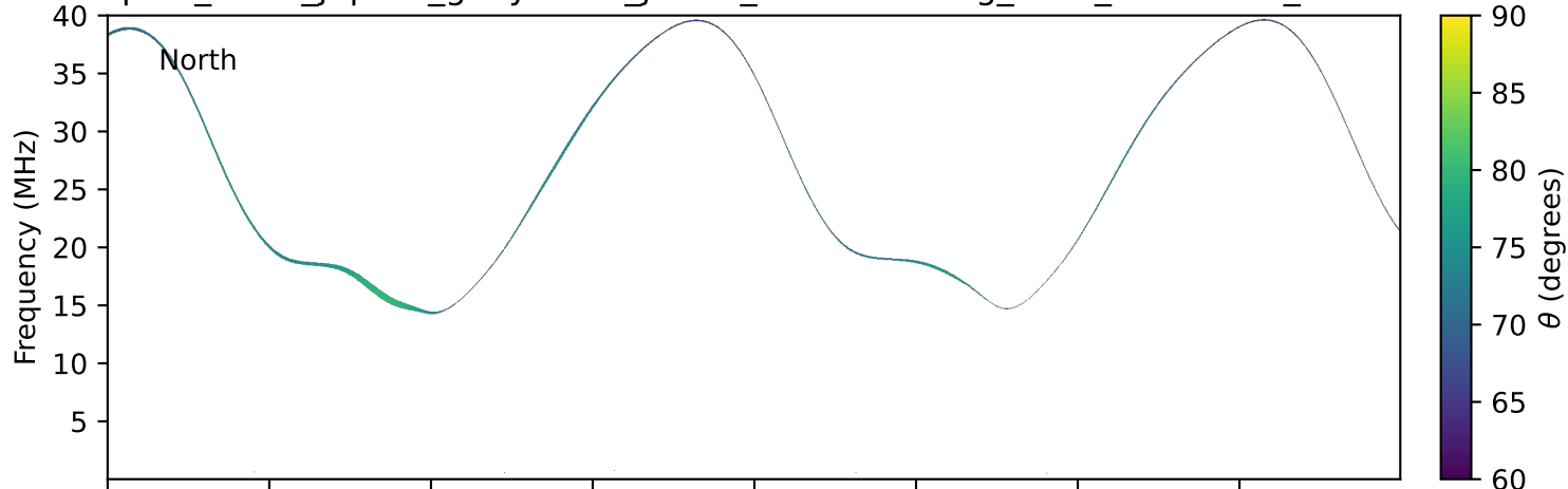
expres_earth_jupiter_ganymede_jrm33_lossc-wid1deg_3kev_19931105_v11.cdf
