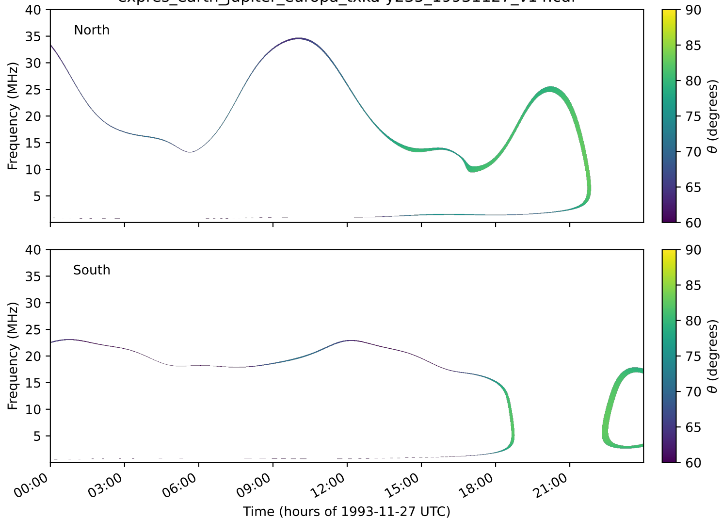
expres_earth_jupiter_europa_txka-y235_19931127_v14.cdf
