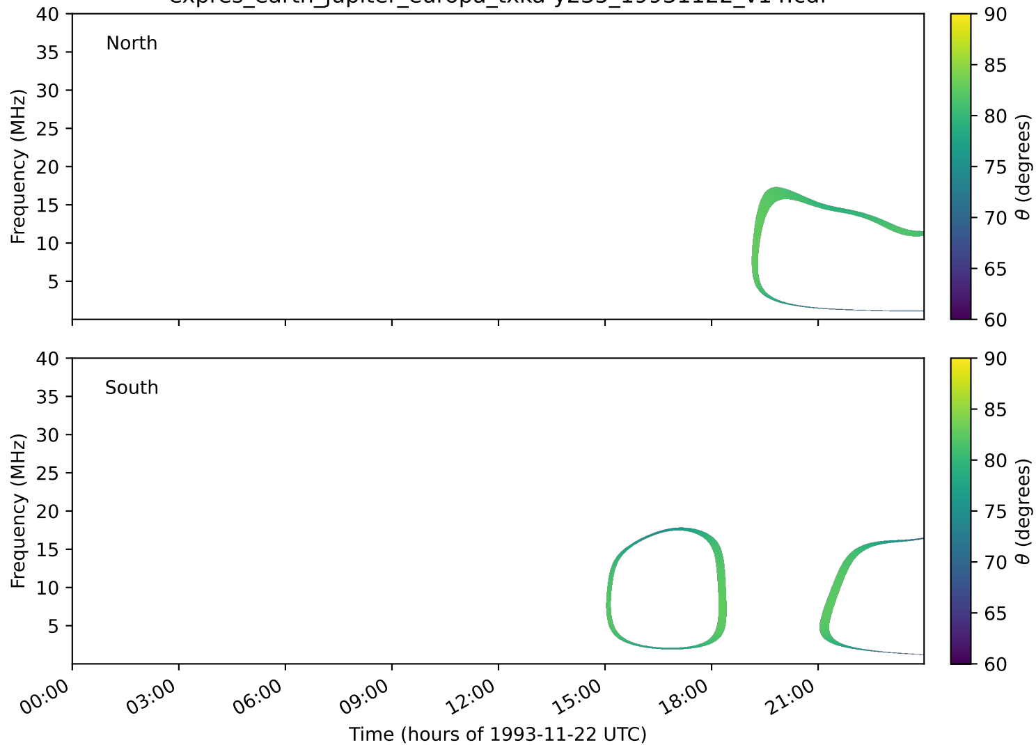
expres_earth_jupiter_europa_txka-y235_19931122_v14.cdf
