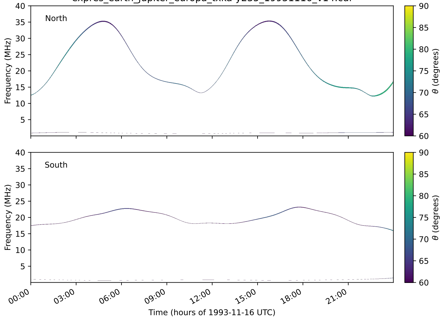
expres_earth_jupiter_europa_txka-y235_19931116_v14.cdf
