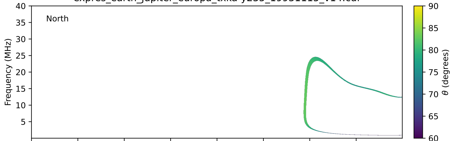
expres_earth_jupiter_europa_txka-y235_19931115_v14.cdf
