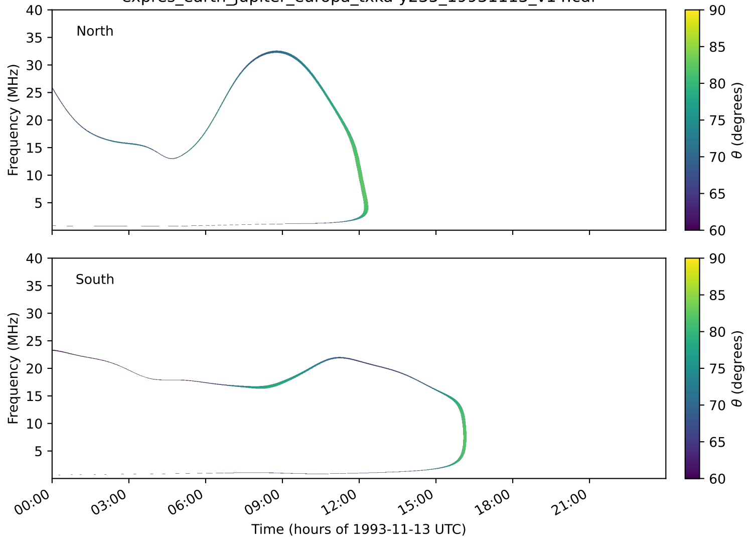
expres_earth_jupiter_europa_txka-y235_19931113_v14.cdf
