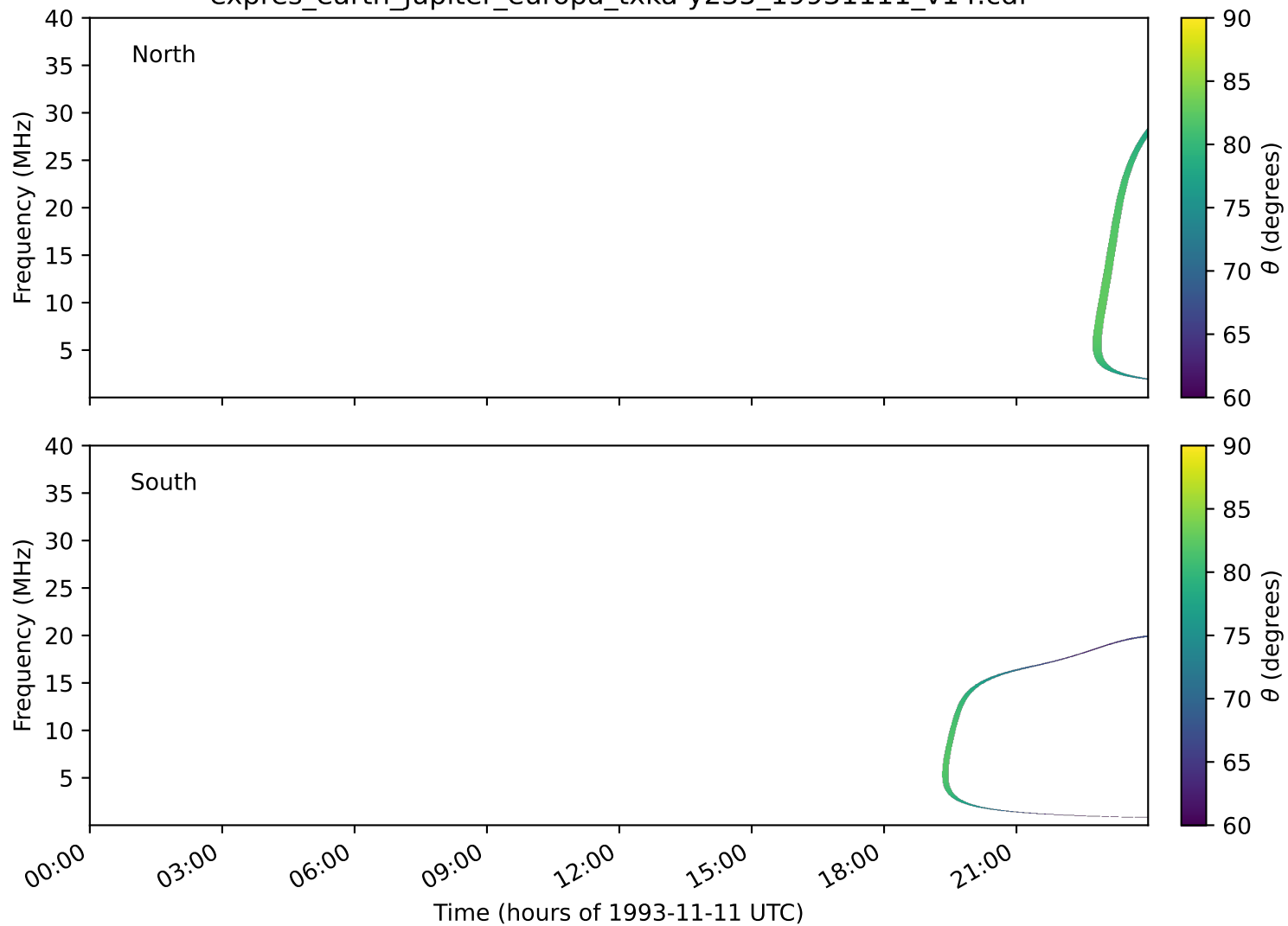
expres_earth_jupiter_europa_txka-y235_19931111_v14.cdf
