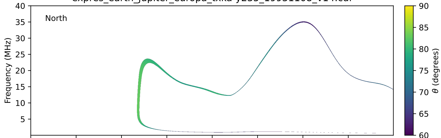
expres_earth_jupiter_europa_txka-y235_19931108_v14.cdf
