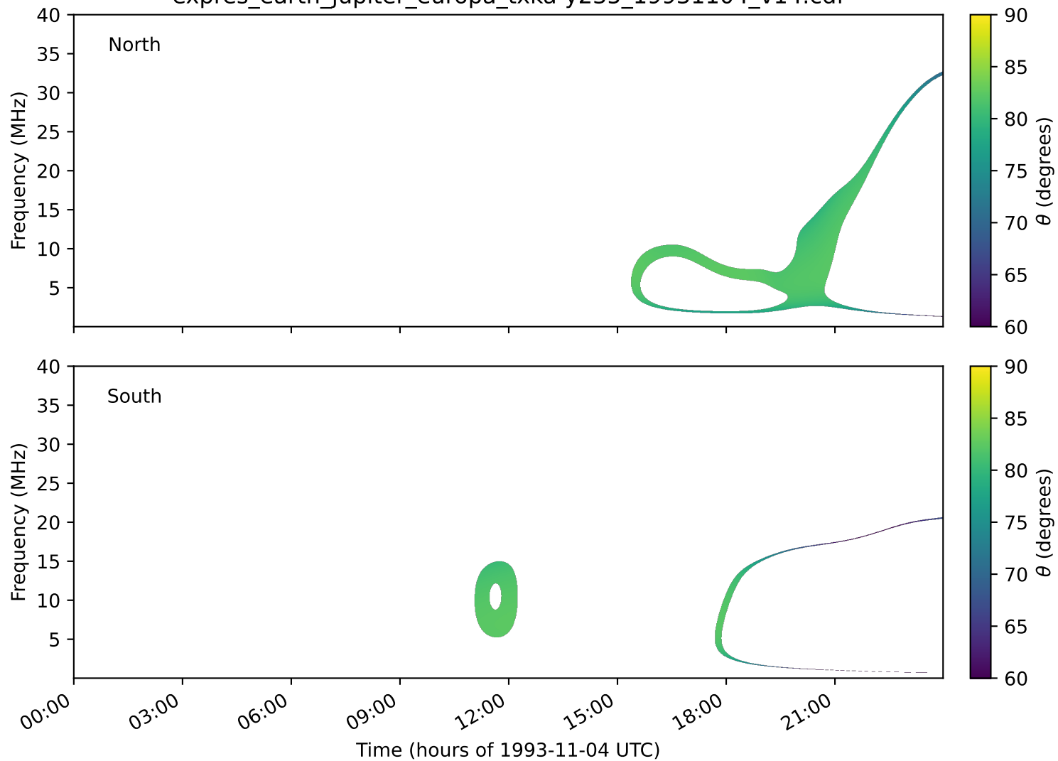
expres_earth_jupiter_europa_txka-y235_19931104_v14.cdf
