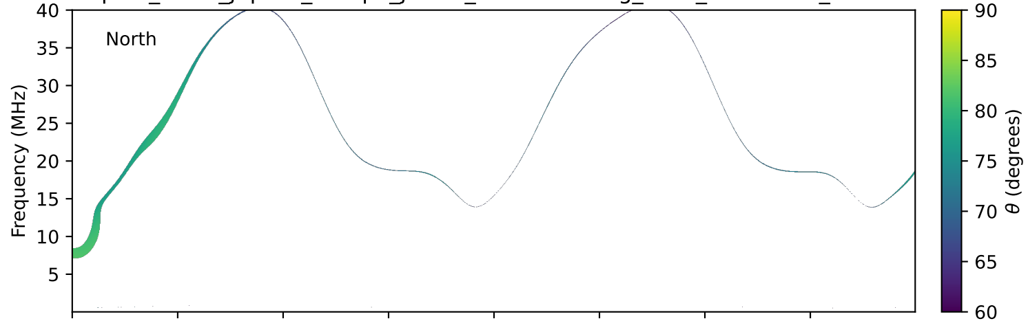
expres_earth_jupiter_europa_jrm33_lossc-wid1deg_3kev_19931123_v11.cdf
