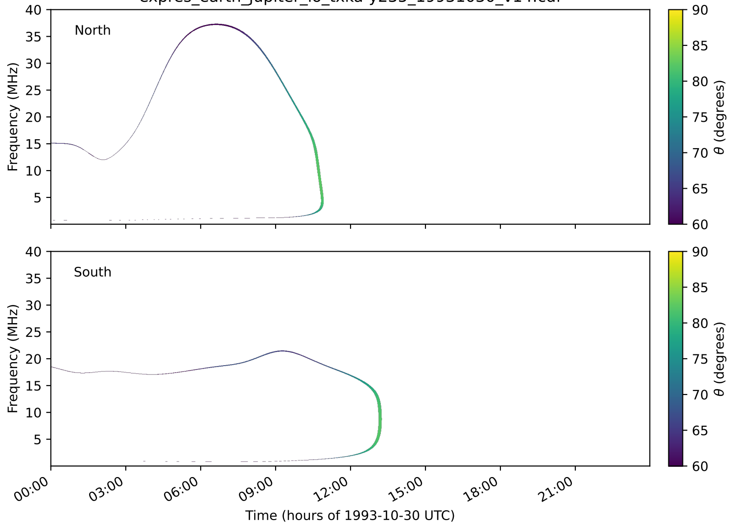
expres_earth_jupiter_io_txka-y235_19931030_v14.cdf
