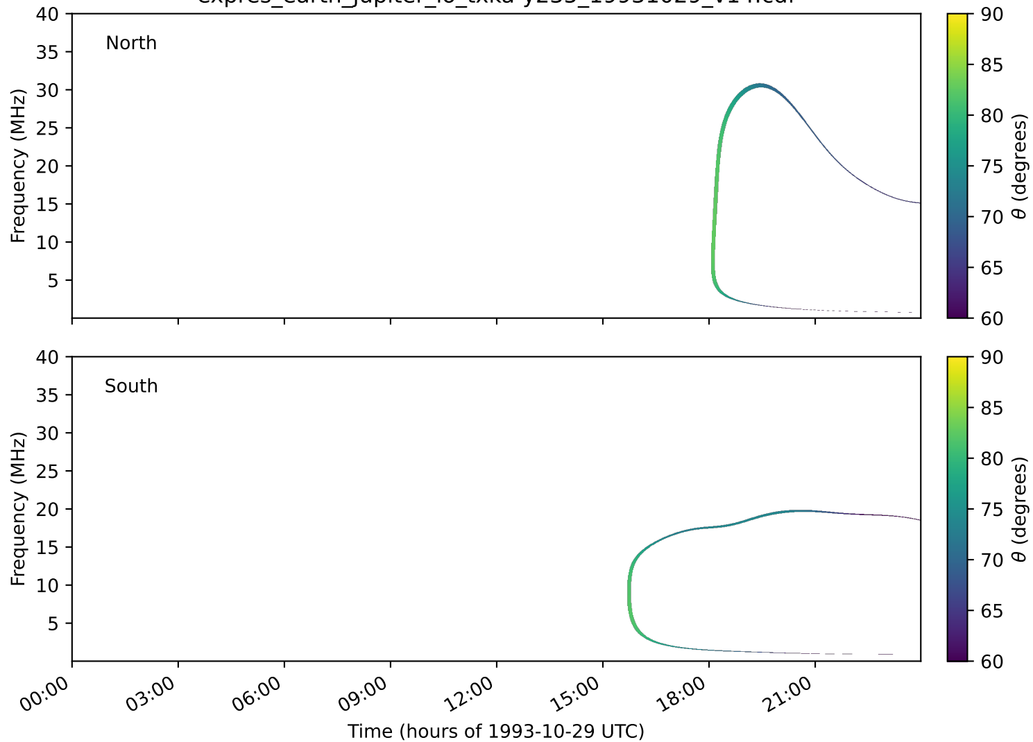
expres_earth_jupiter_io_txka-y235_19931029_v14.cdf
