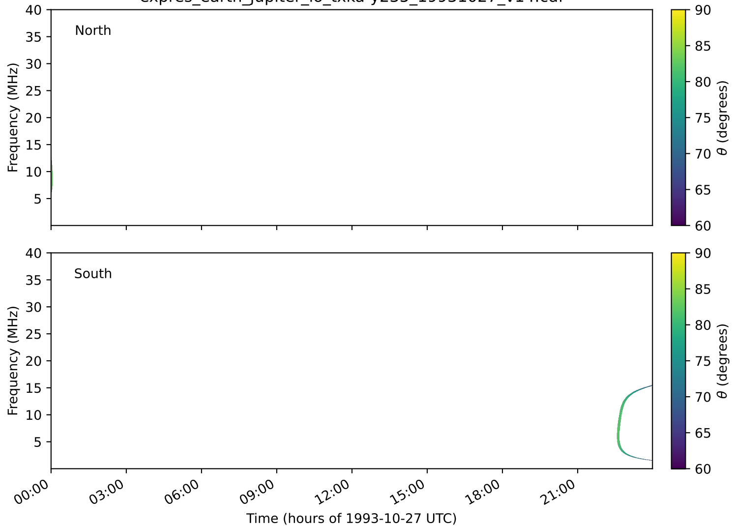
expres_earth_jupiter_io_txka-y235_19931027_v14.cdf
