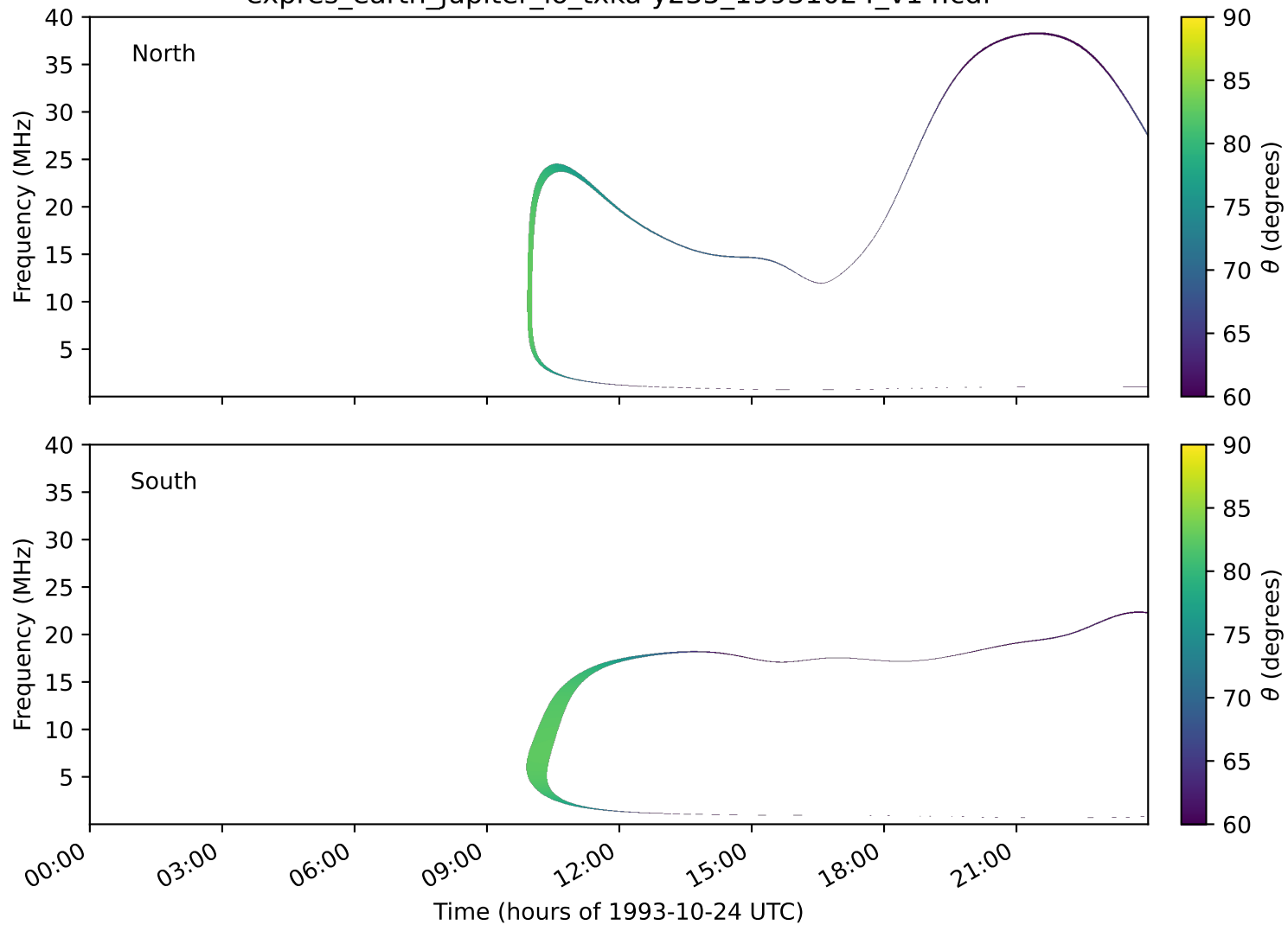
expres_earth_jupiter_io_txka-y235_19931024_v14.cdf
