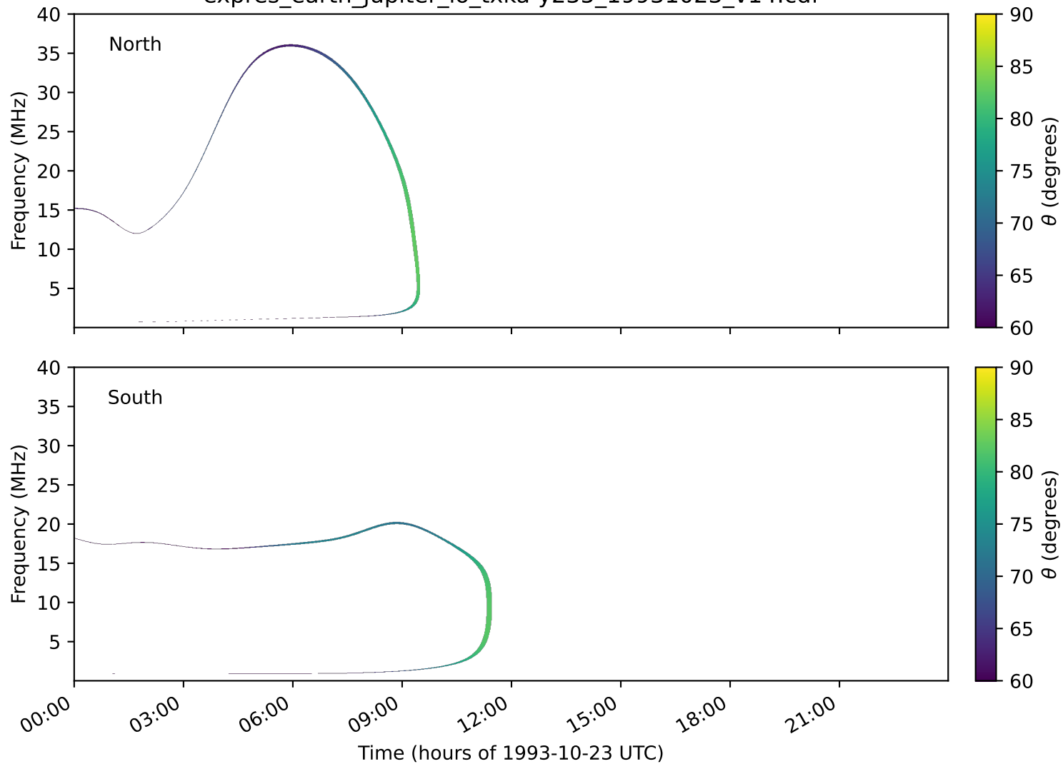
expres_earth_jupiter_io_txka-y235_19931023_v14.cdf
