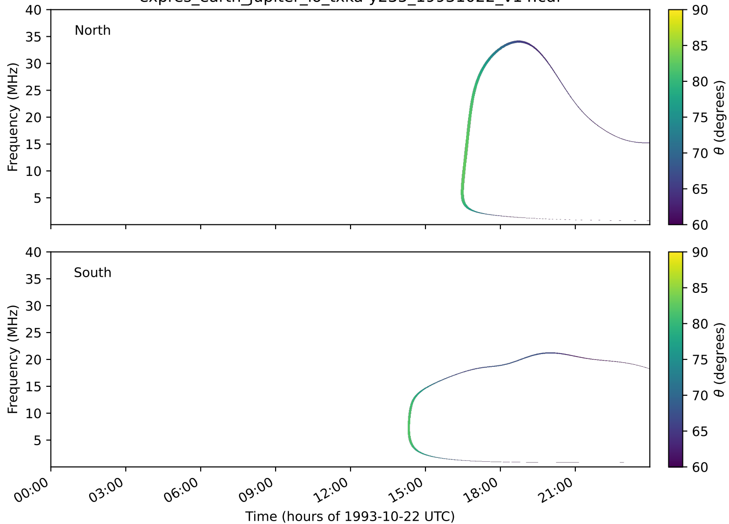
expres_earth_jupiter_io_txka-y235_19931022_v14.cdf
