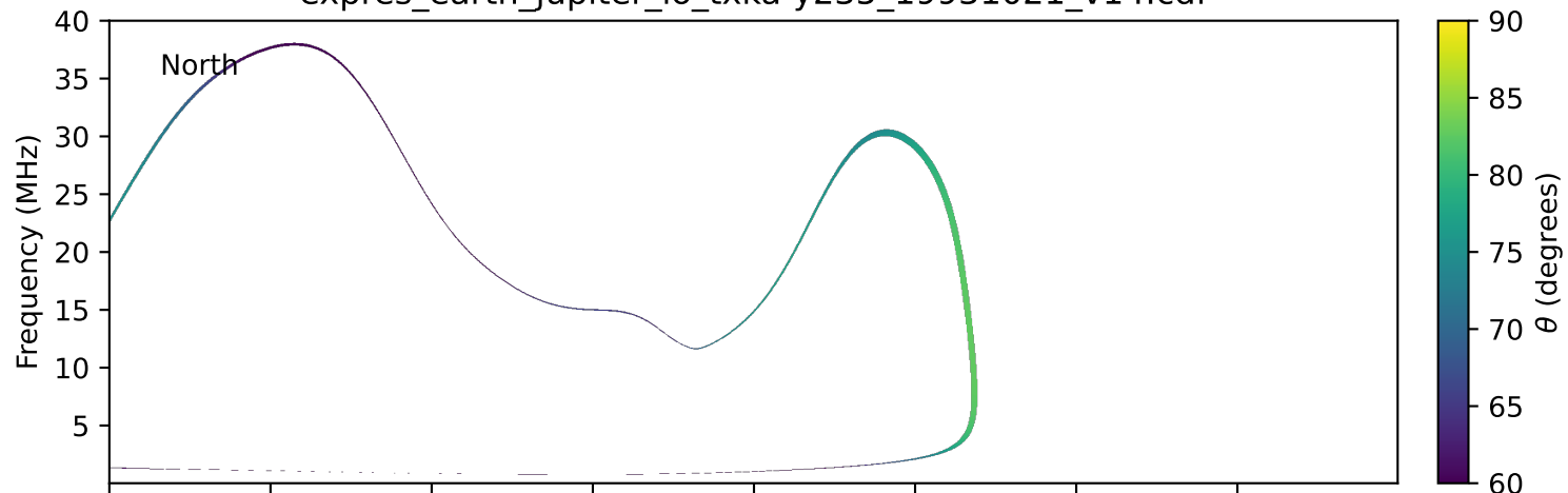
expres_earth_jupiter_io_txka-y235_19931021_v14.cdf
