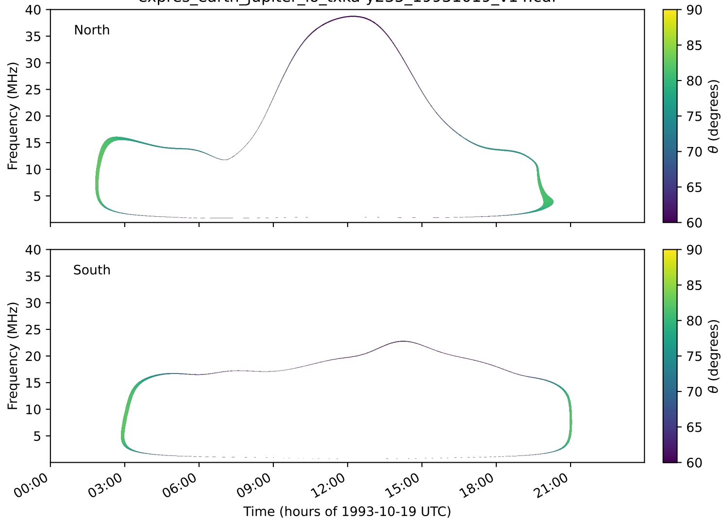
expres_earth_jupiter_io_txka-y235_19931019_v14.cdf
