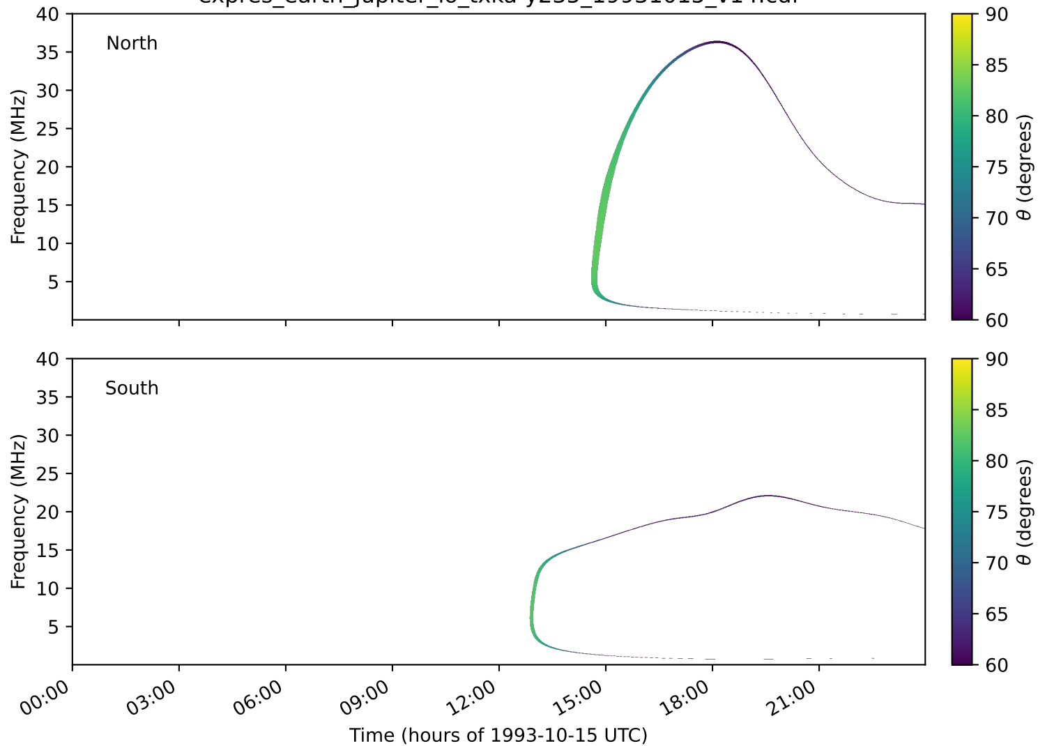
expres_earth_jupiter_io_txka-y235_19931015_v14.cdf
