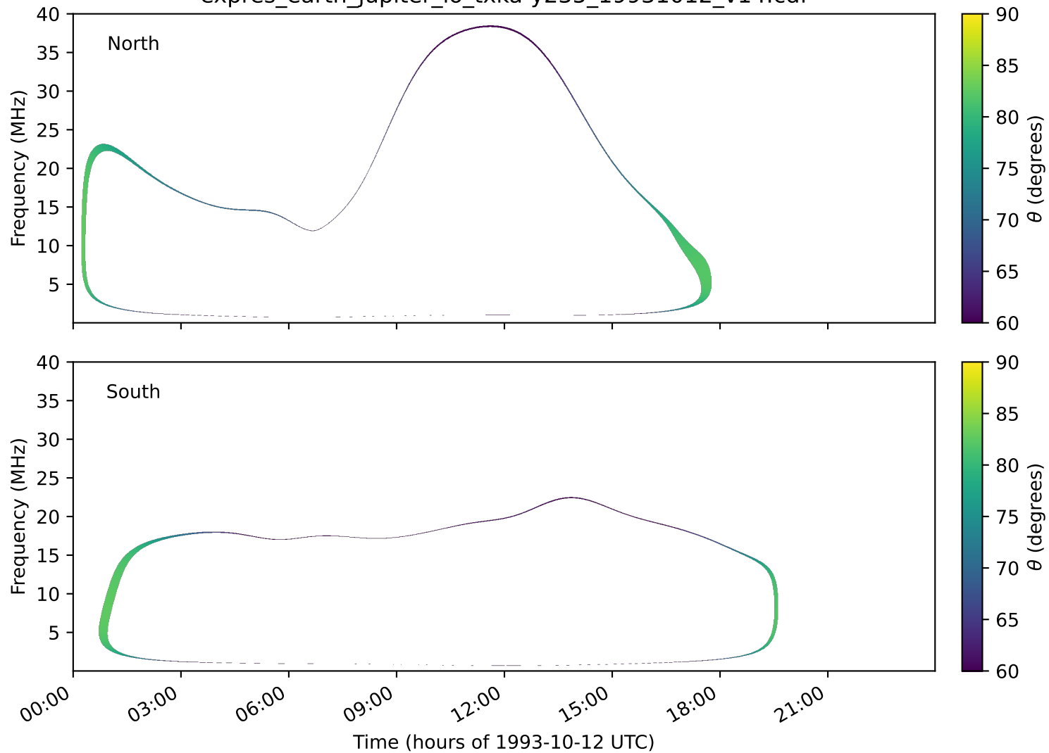
expres_earth_jupiter_io_txka-y235_19931012_v14.cdf
