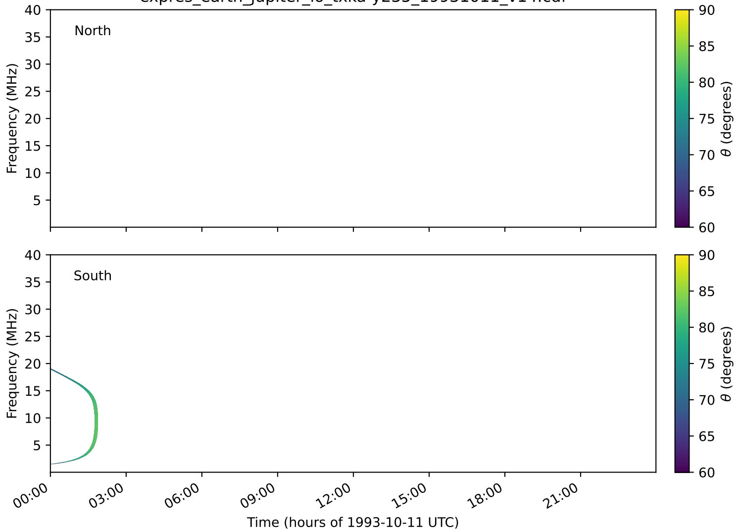
expres_earth_jupiter_io_txka-y235_19931011_v14.cdf
