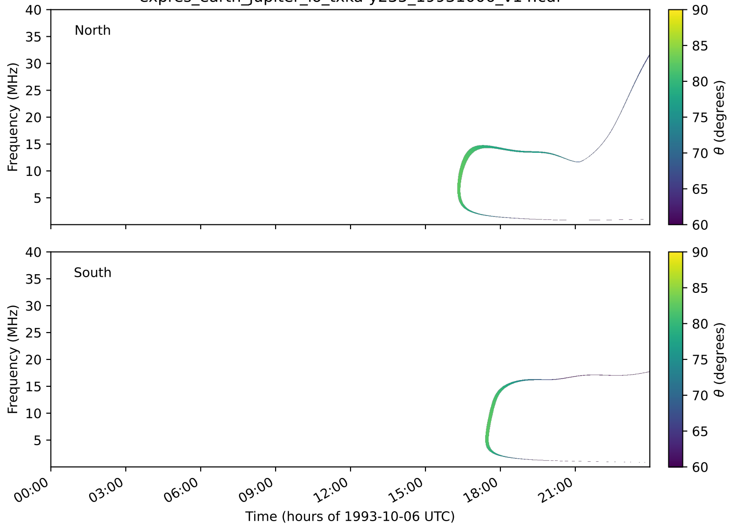
expres_earth_jupiter_io_txka-y235_19931006_v14.cdf
