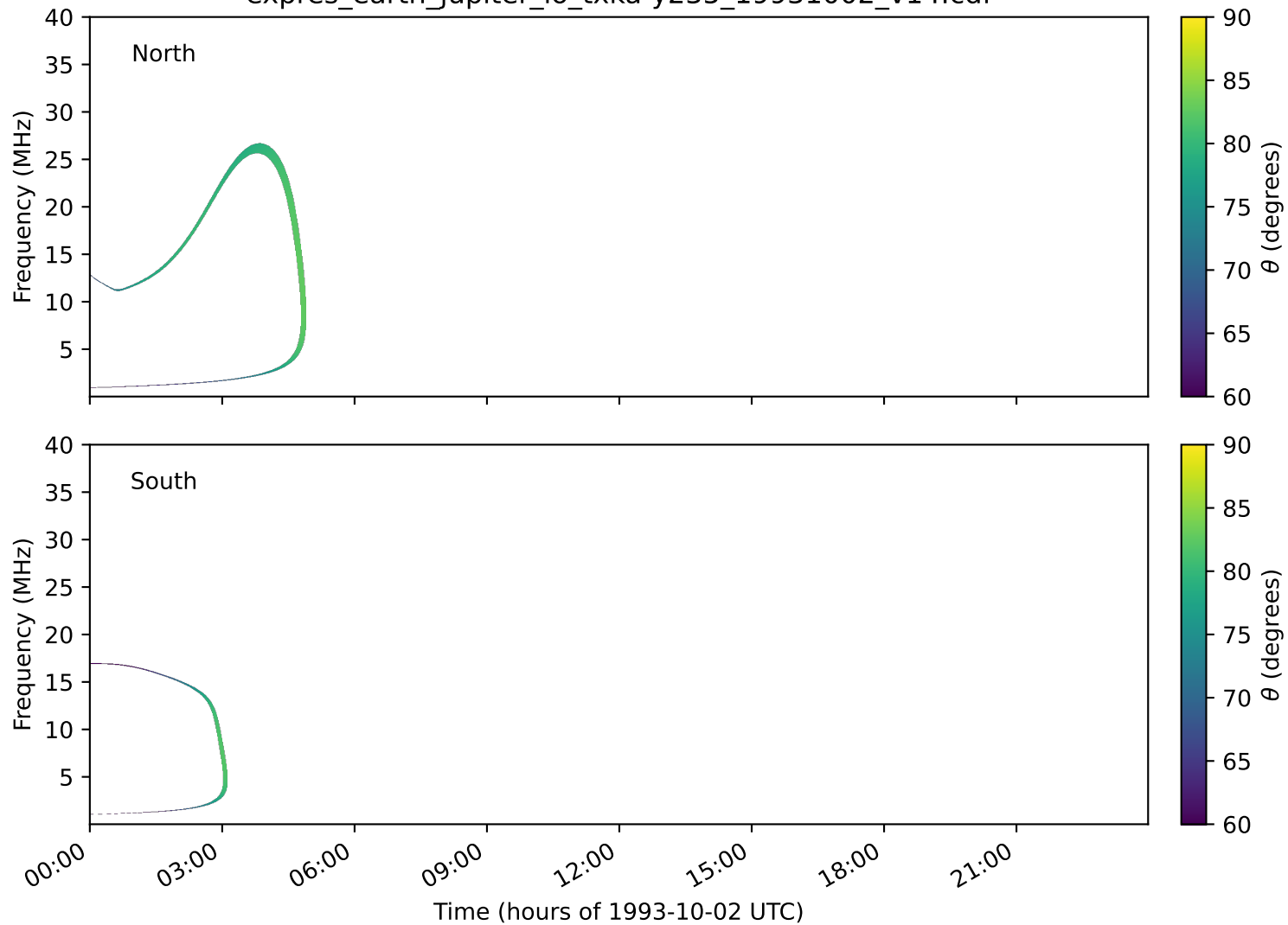
expres_earth_jupiter_io_txka-y235_19931002_v14.cdf
