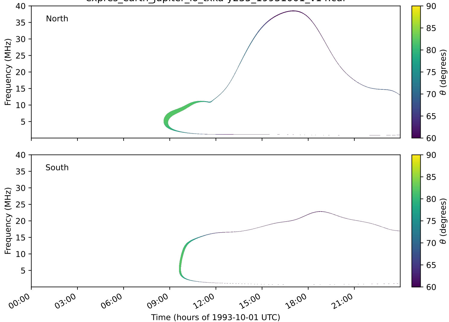
expres_earth_jupiter_io_txka-y235_19931001_v14.cdf
