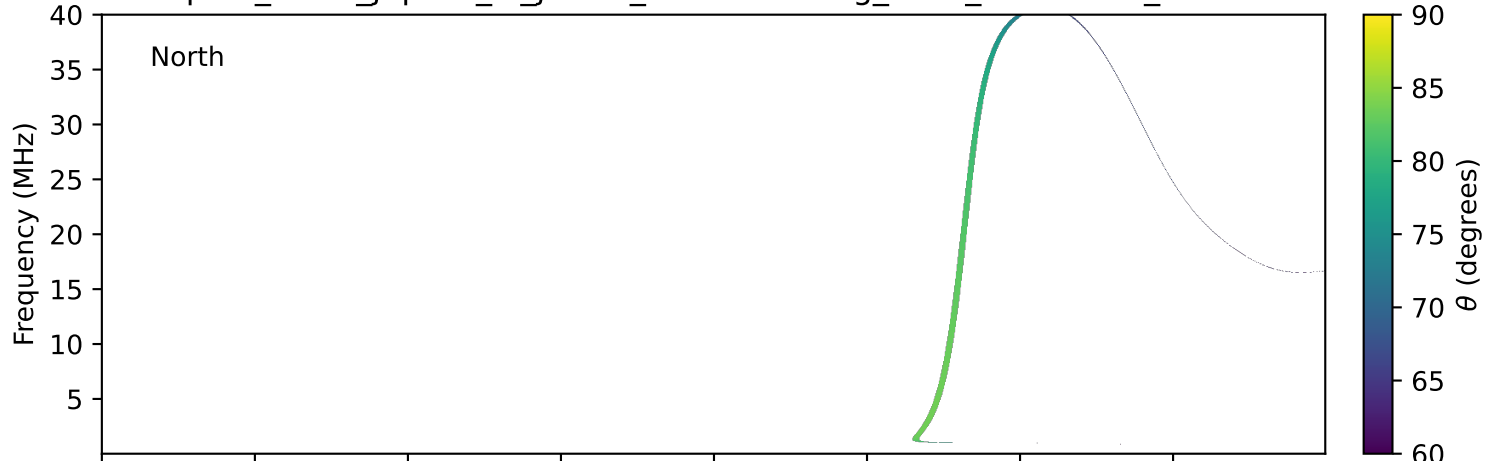
expres_earth_jupiter_io_jrm33_lossc-wid1deg_3kev_19931022_v11.cdf
