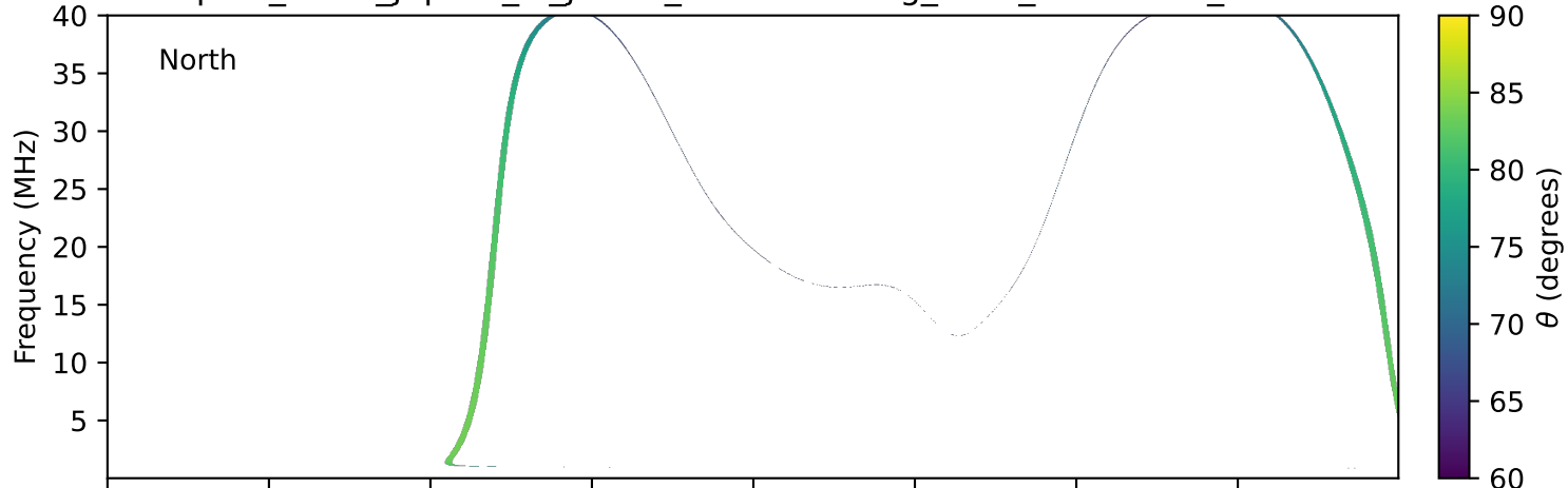
expres_earth_jupiter_io_jrm33_lossc-wid1deg_3kev_19931010_v11.cdf
