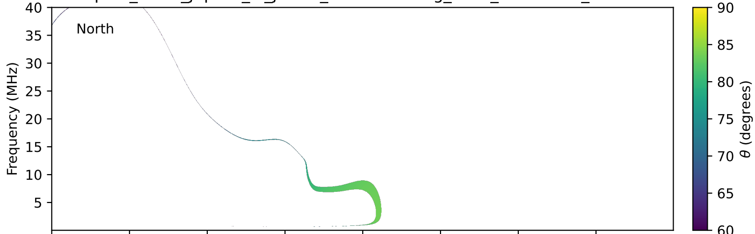
expres_earth_jupiter_io_jrm33_lossc-wid1deg_3kev_19931007_v11.cdf
