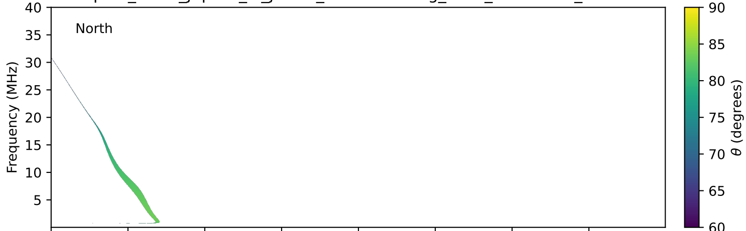
expres_earth_jupiter_io_jrm09_lossc-wid1deg_3kev_19931025_v11.cdf
