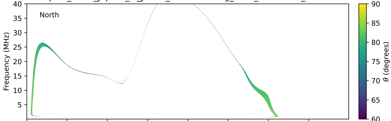
expres_earth_jupiter_io_jrm09_lossc-wid1deg_3kev_19931012_v11.cdf
