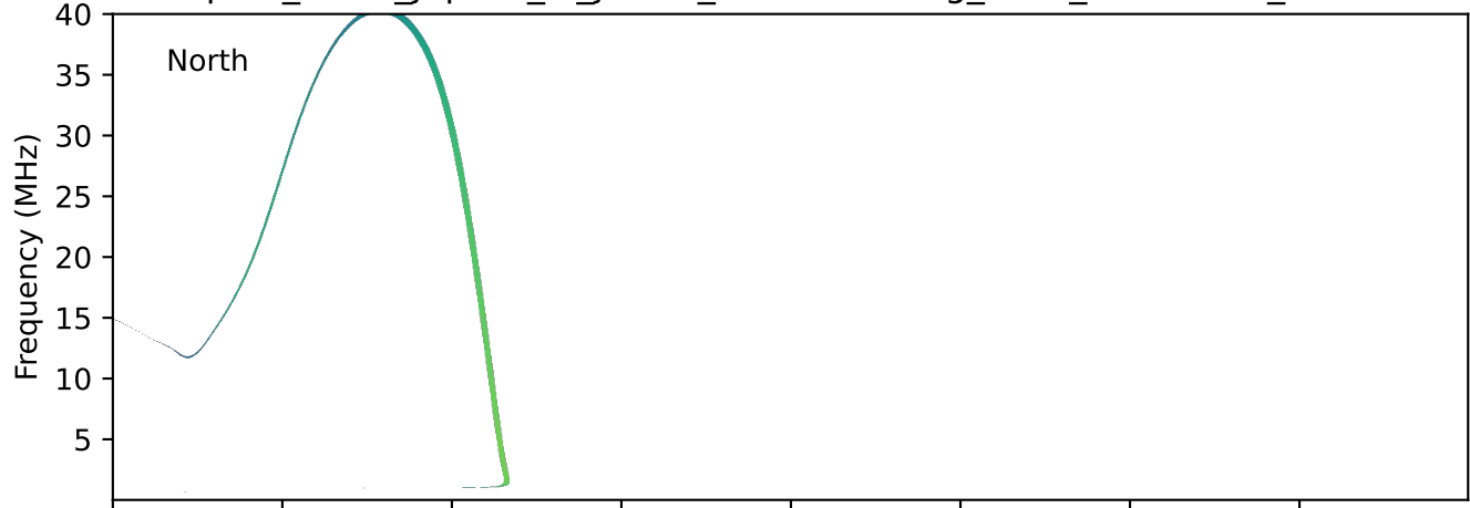
expres_earth_jupiter_io_jrm09_lossc-wid1deg_3kev_19931009_v11.cdf
