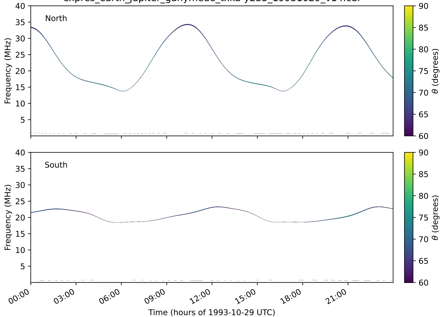
expres_earth_jupiter_ganymede_txka-y235_19931029_v14.cdf
