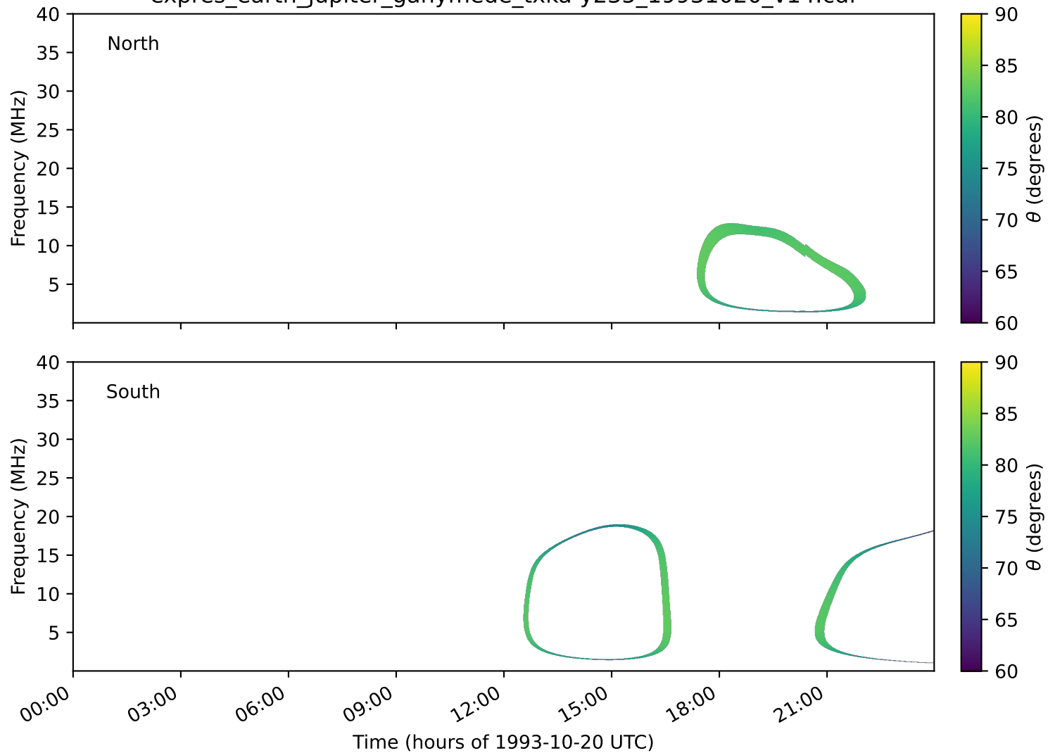
expres_earth_jupiter_ganymede_txka-y235_19931020_v14.cdf
