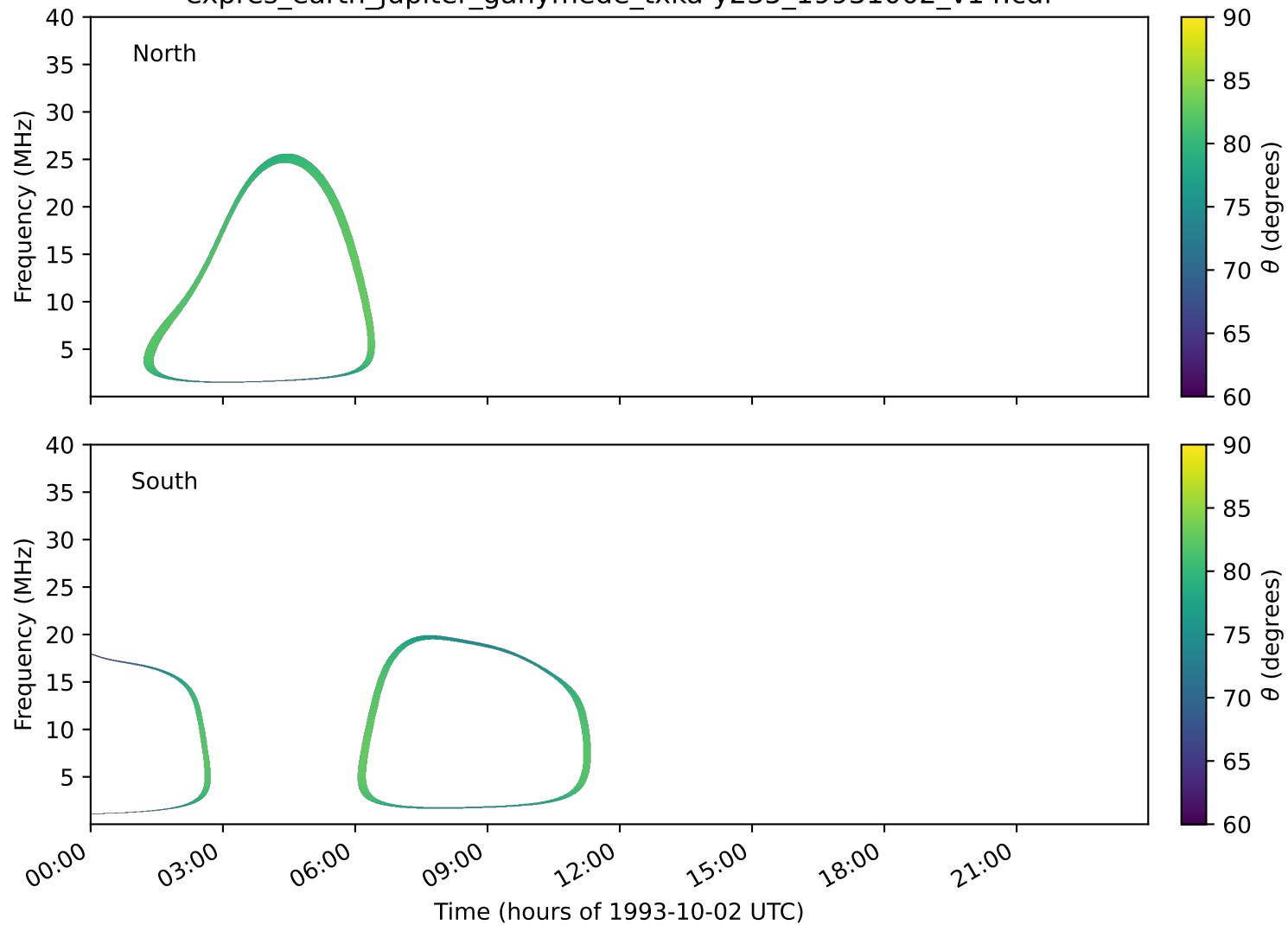
expres_earth_jupiter_ganymede_txka-y235_19931002_v14.cdf
